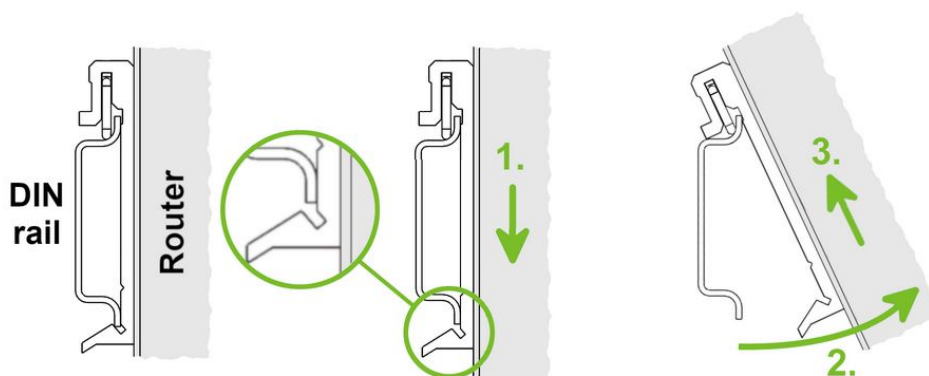
Figure 5: Removing the router from the DIN rail
