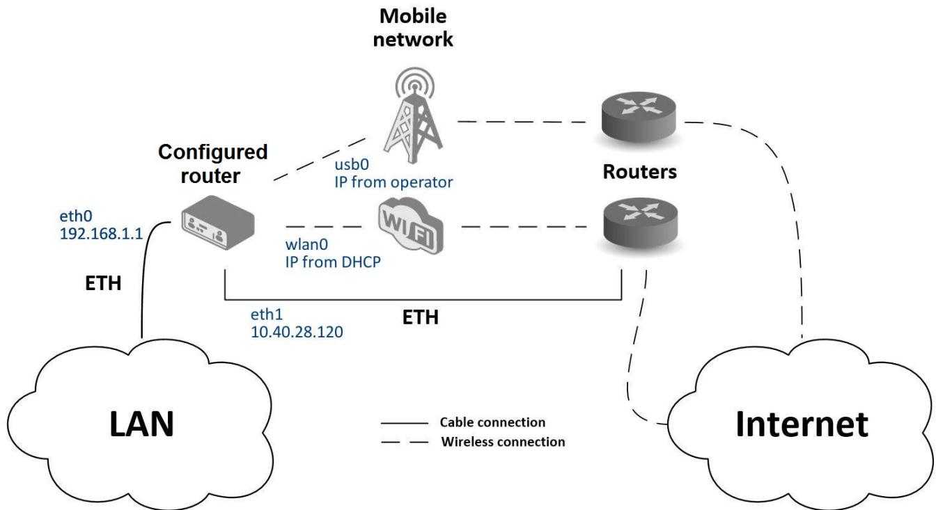
Figure 122: Backup access to the internet: a topology example
