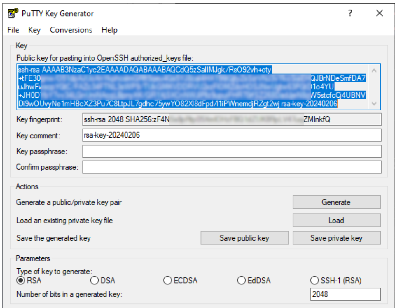
Figure 102: Generating an RSA key pair with PuTTYgen
