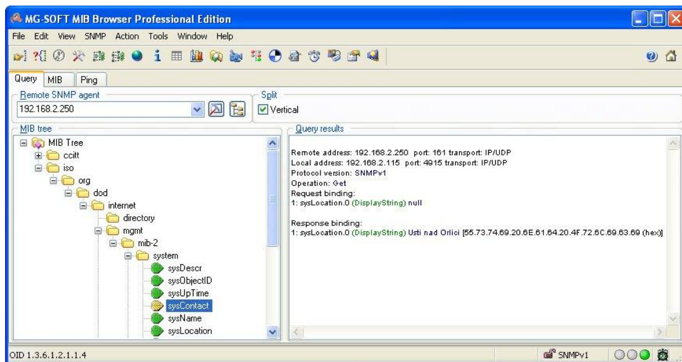
Figure 82: MIB browser example
