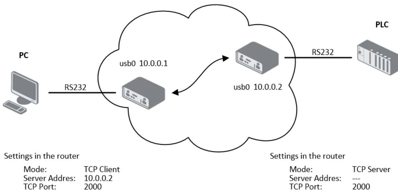
Figure 85: Serial interface configuration example
