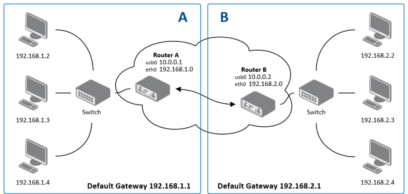
Figure 61: IPsec configuration topology example
