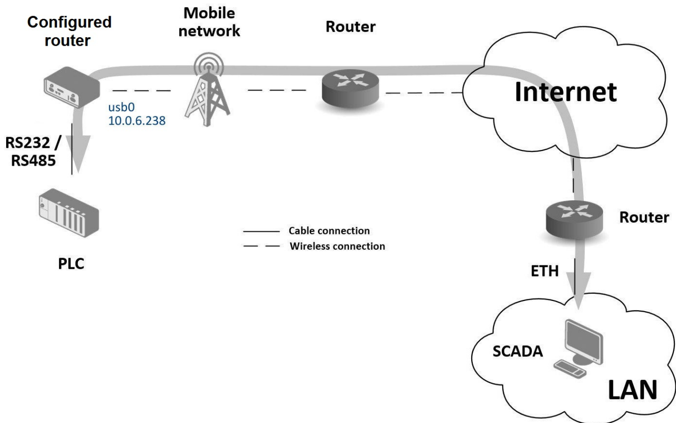
Figure 125: Serial gateway: a topology example
