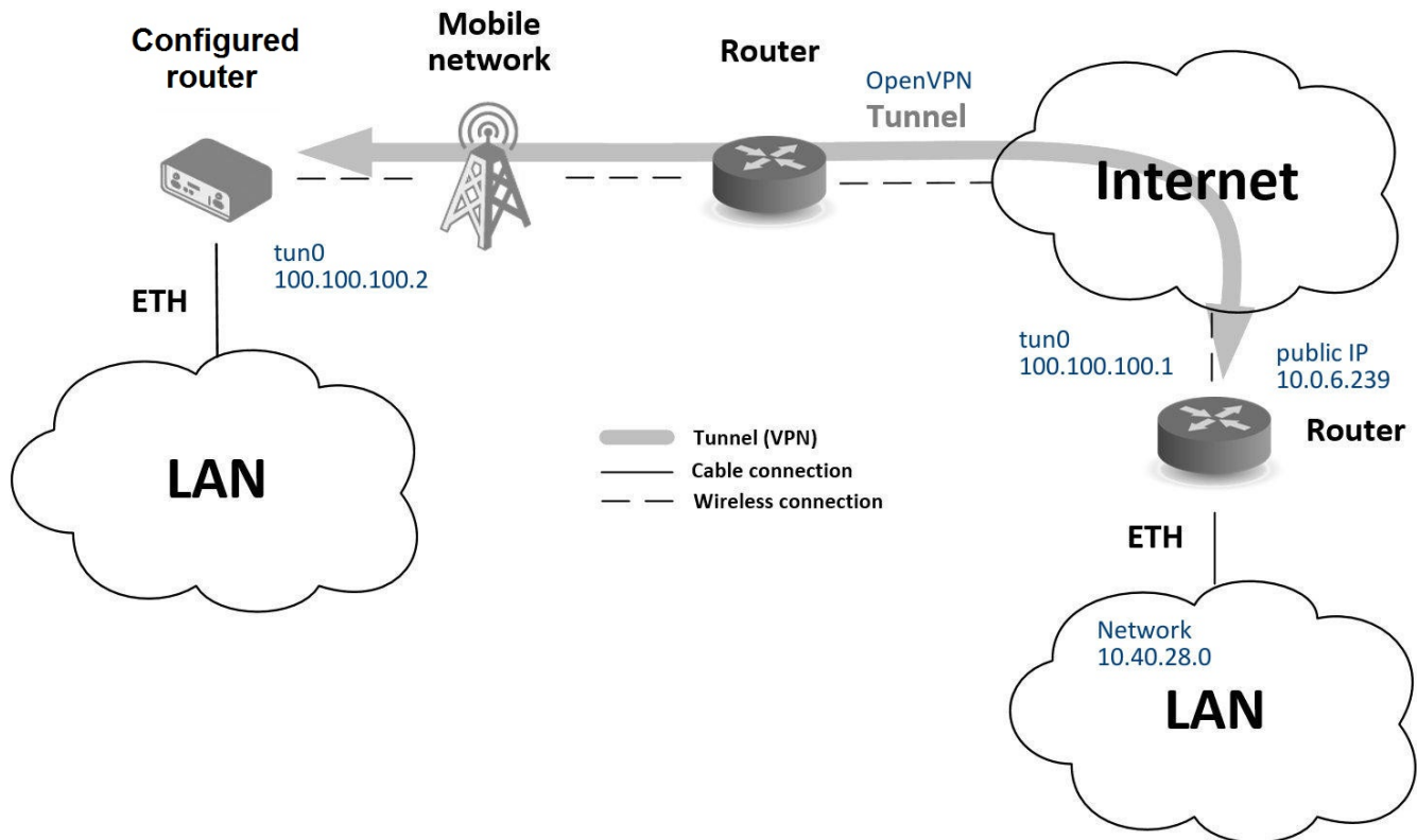
Figure 123: Secure networks interconnection: a topology example
