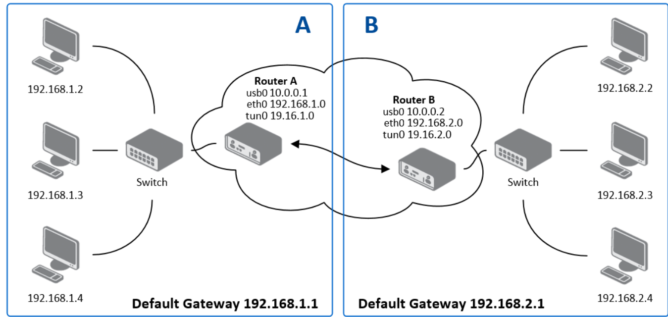
Figure 58: An example of OpenVPN topology
