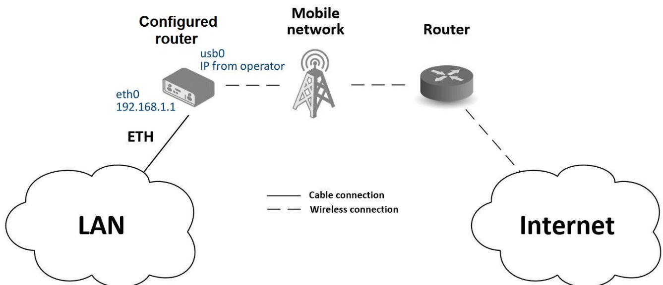
Figure 115: Access to the internet from LAN: a topology example
