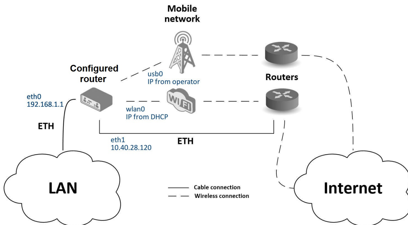
Figure 118: Backup access to the internet: a topology example
