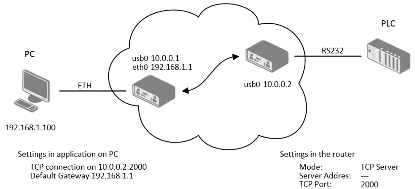
Figure 84: Ethernet-to-serial communication configuration example
