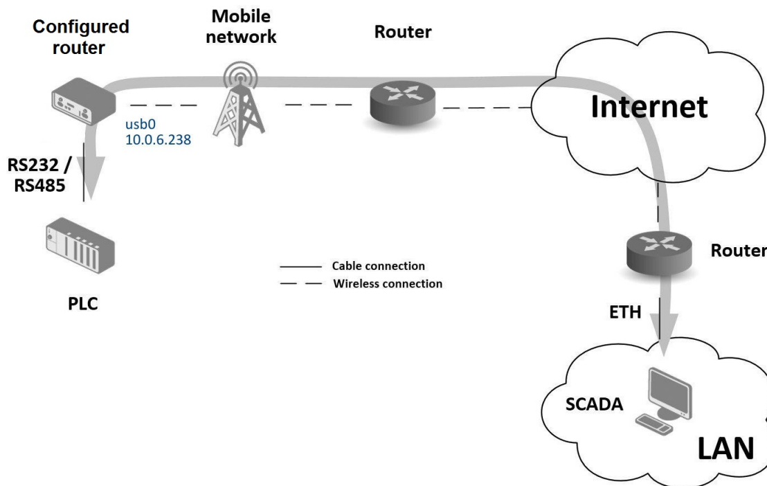
Figure 126: Serial Gateway – sample topology
