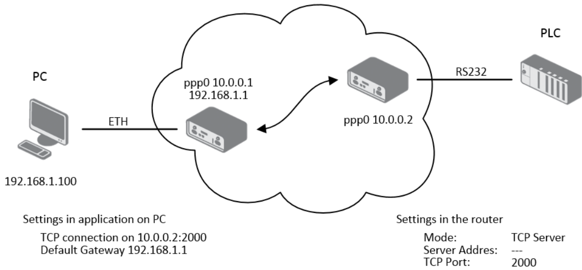
Figure 84: Example of Ethernet to serial communication configuration
