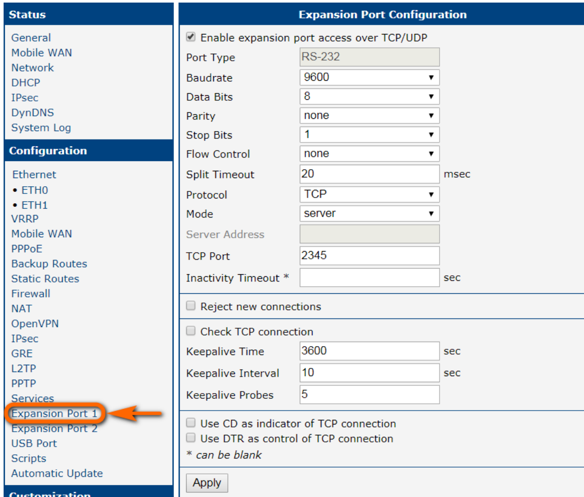
Figure 126: Serial Gateway – konfigurace Expansion Port 1
