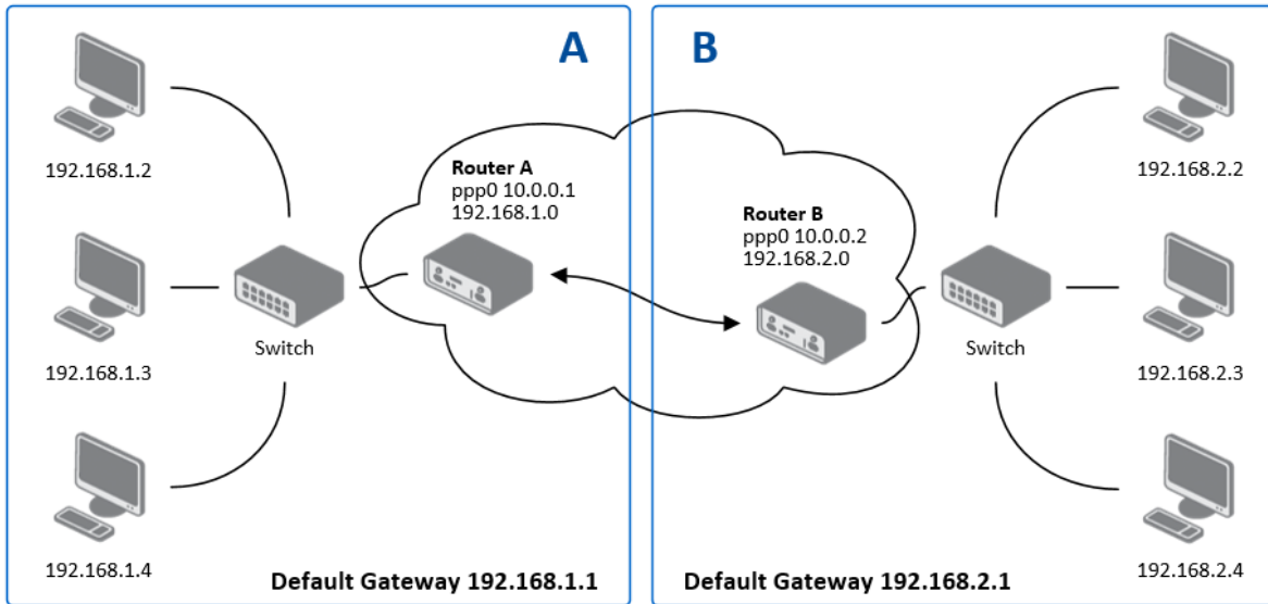
Figure 56: Topology of IPsec Configuration Example
