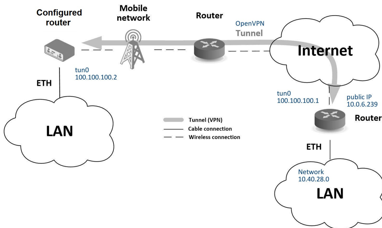
Figure 126: Secure networks interconnection: a topology example
