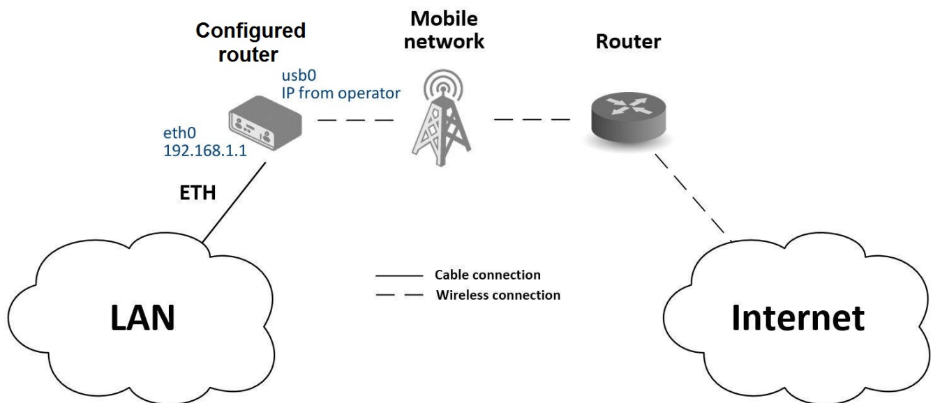
Figure 118: Access to the internet from LAN: a topology example
