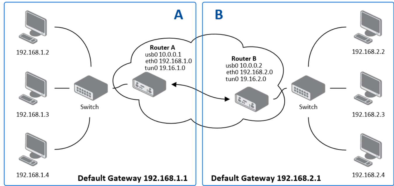
Figure 61: An example of OpenVPN topology
