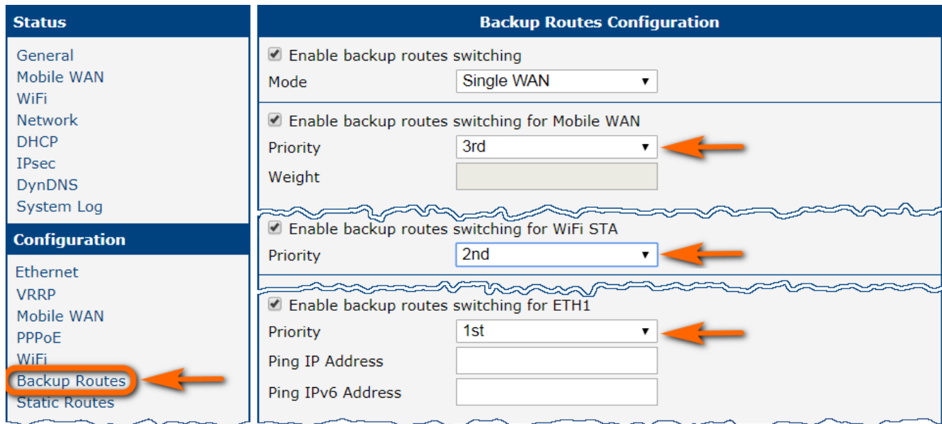
Figure 125: Backup access to the internet: backup routes configuration
