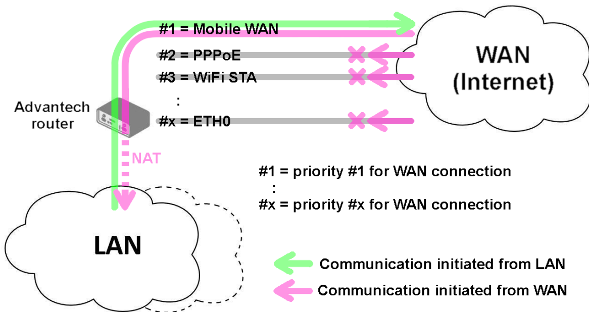
Figure 35: Example #1: Topology
