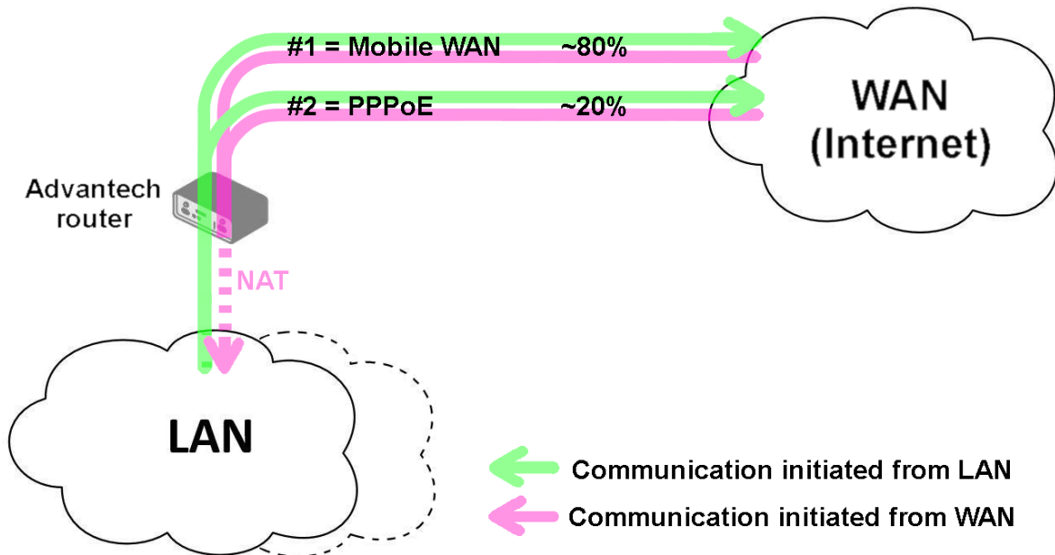
Figure 41: Example #4: Topology
