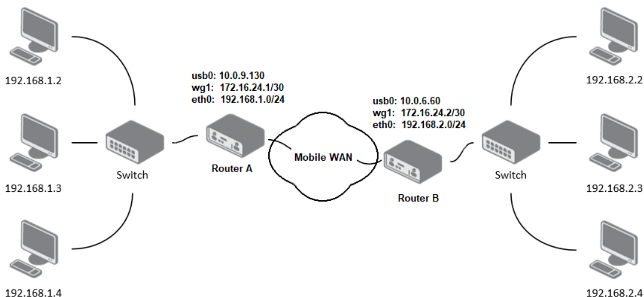
Figure 68: An example of WireGuard topology
