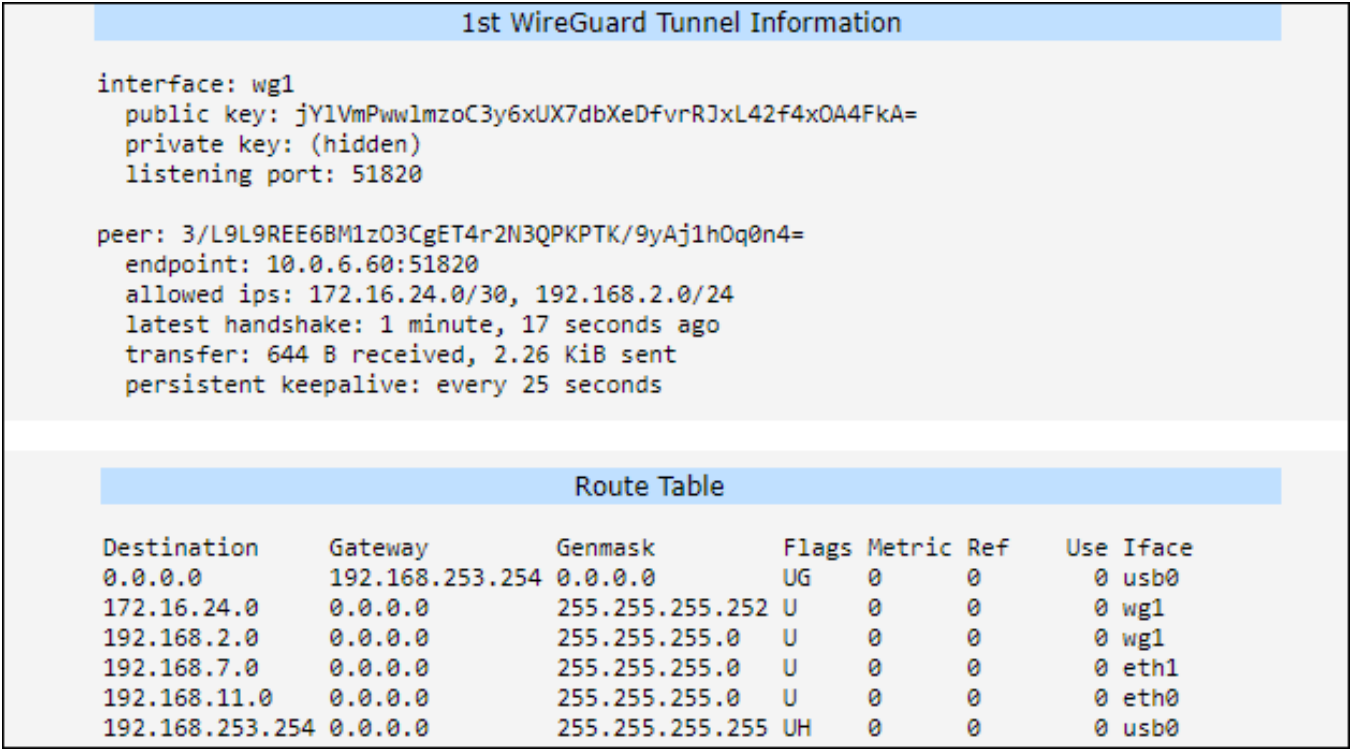
Figure 69: Router A: WireGuard status and route table
