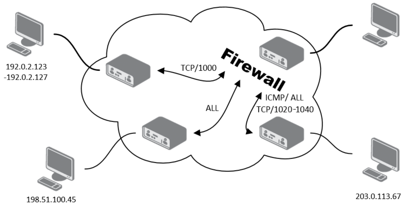
Figure 54: IPv4 firewall configuration topology example
