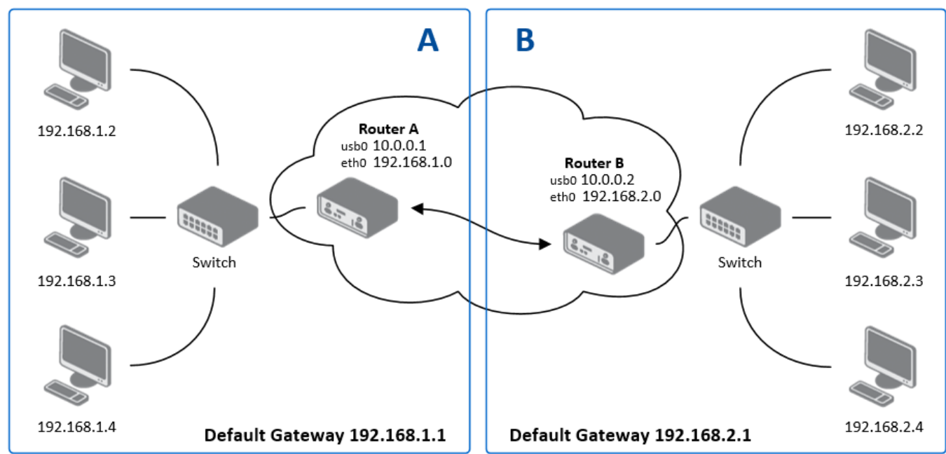
Figure 66: IPsec configuration topology example
