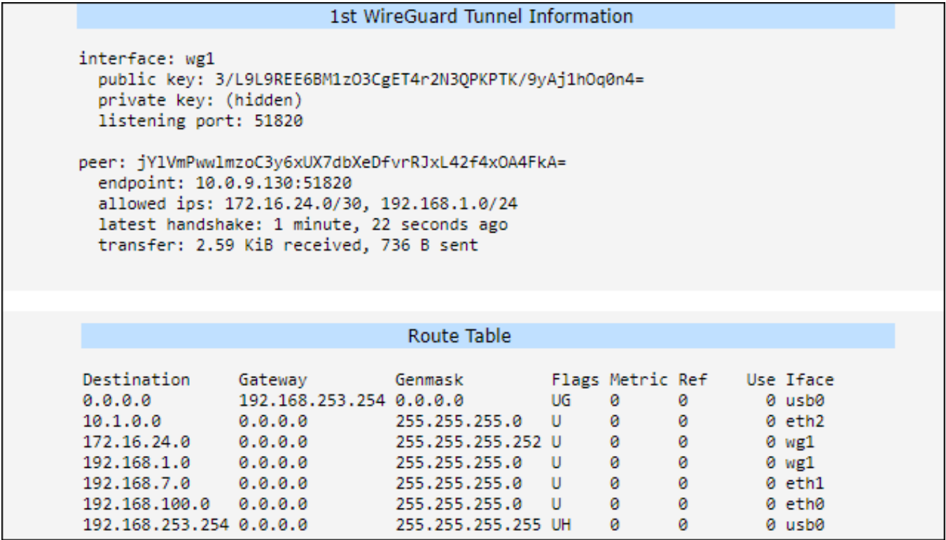
Figure 70: Router B: WireGuard status and route table
