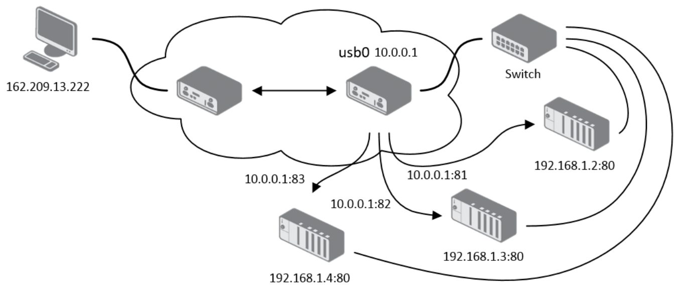
Figure 60: Topology for NAT example 2
