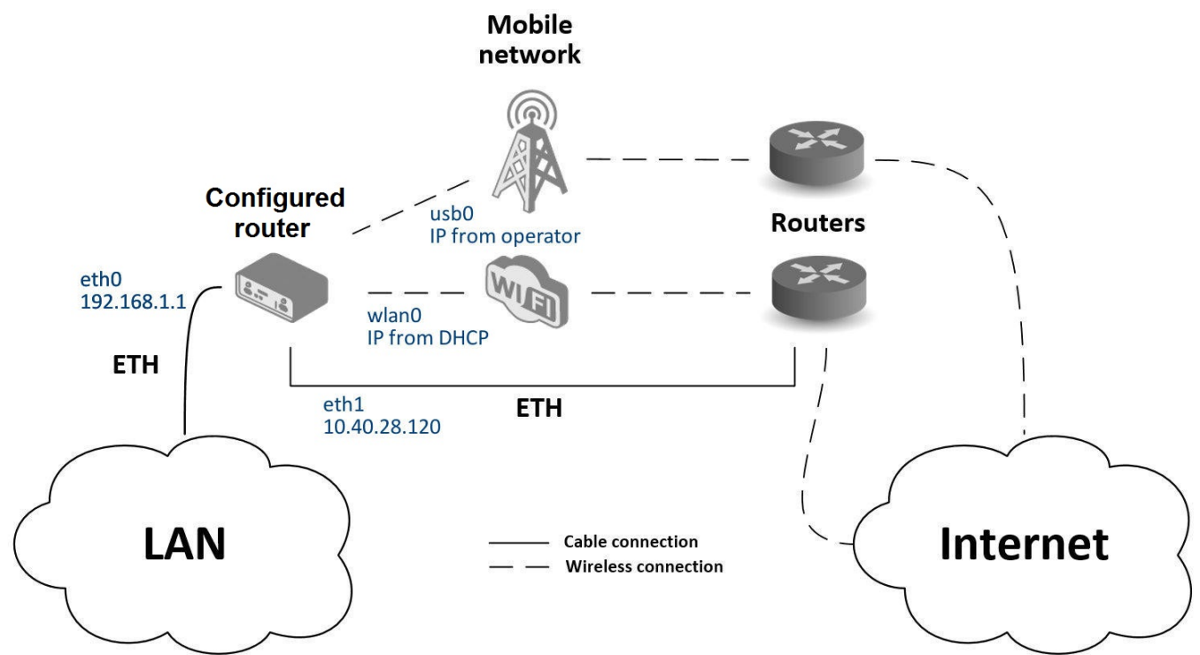
Figure 125: Backup access to the internet – sample topology
