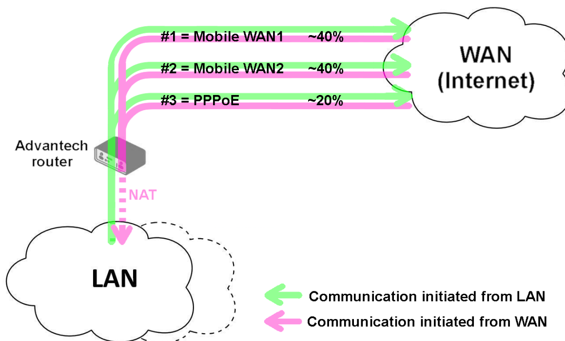
Figure 47: Network topology for example 5
