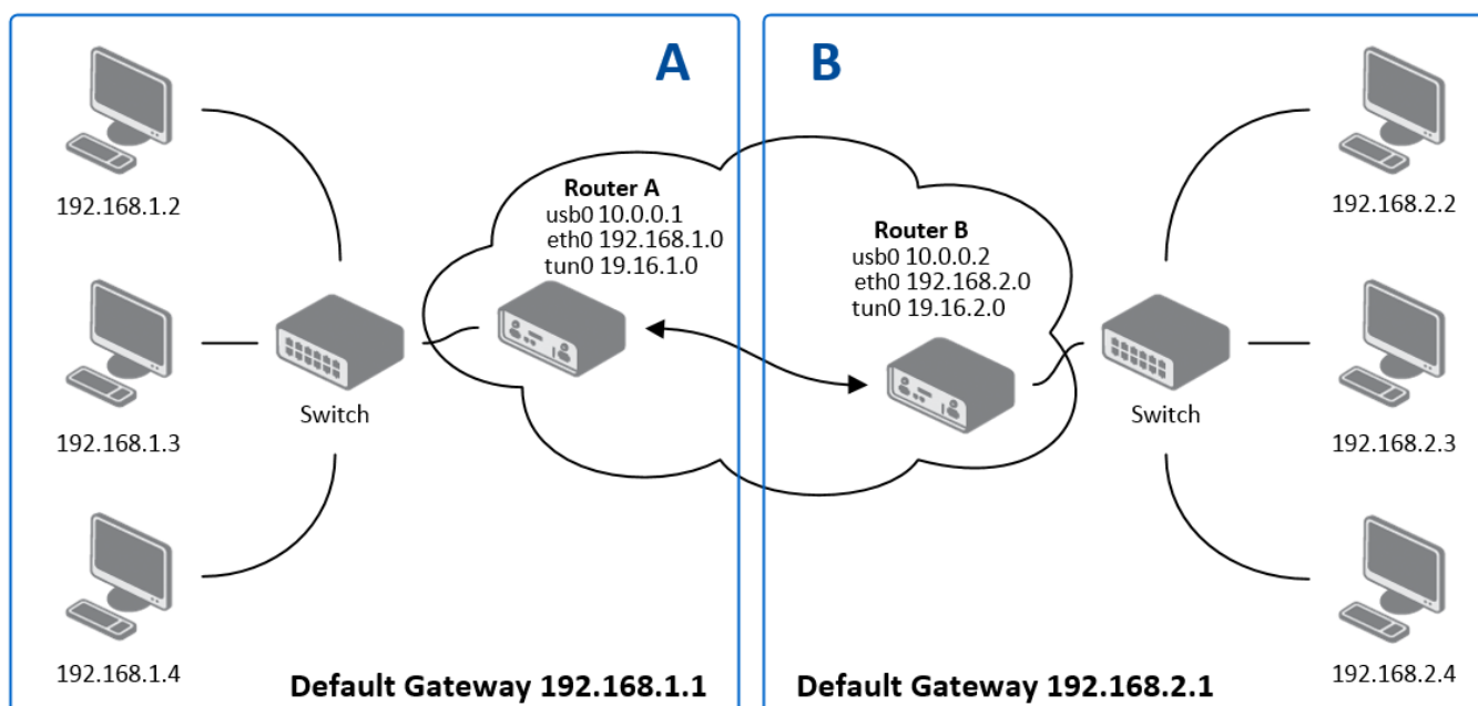
Figure 63: An example of OpenVPN topology
