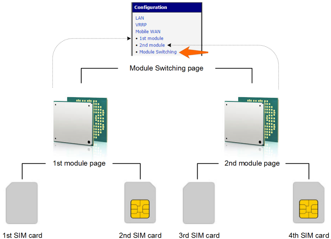
Figure 27: Switching and configuration pages structure
