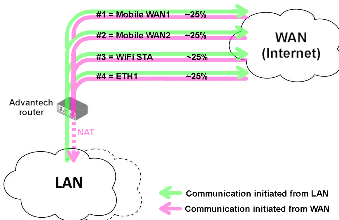
Figure 49: Network topology for example 6
