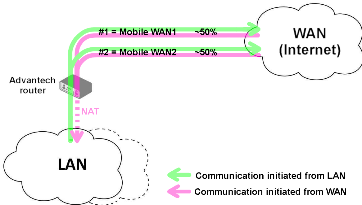
Figure 43: Example #4: Topology
