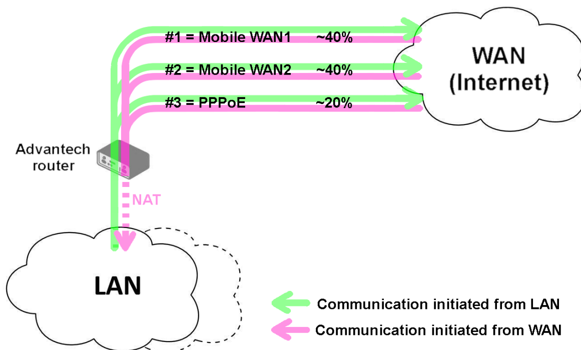
Figure 46: Example #5: Topology
