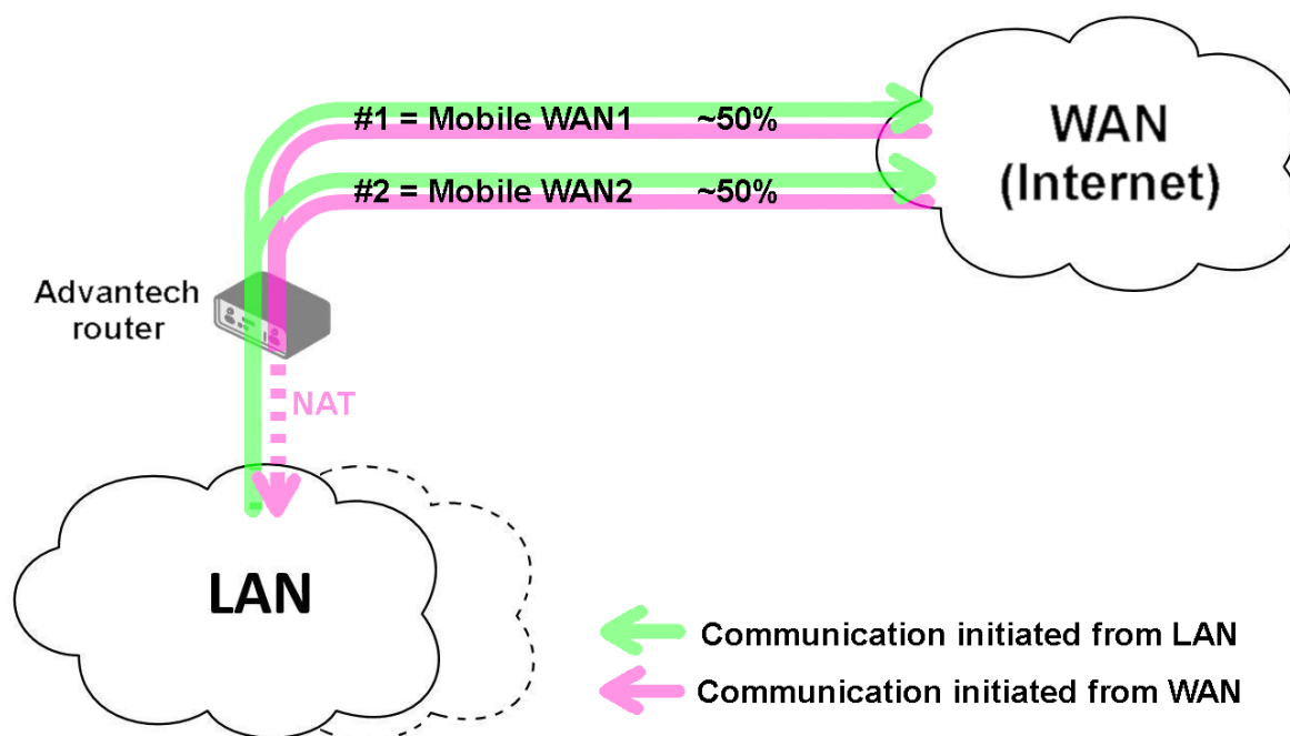
Figure 44: Example #4: Topology
