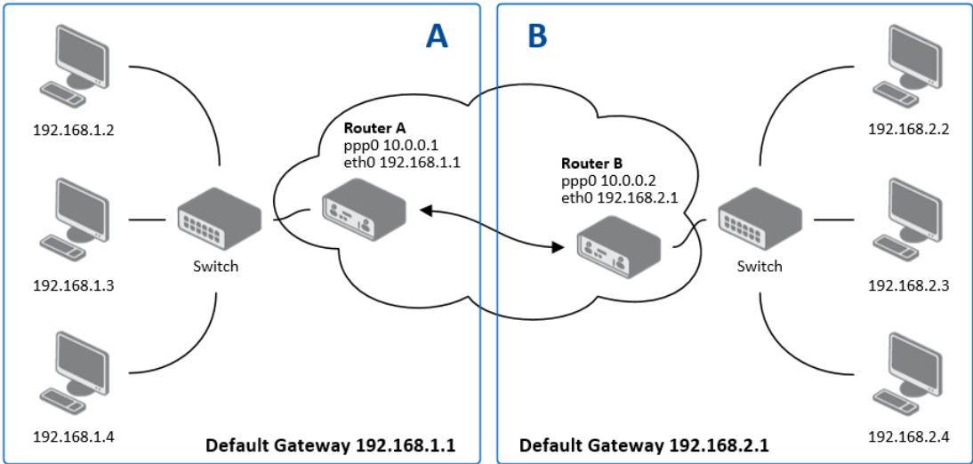
Figure 70: Topology of GRE Tunnel Configuration Example
