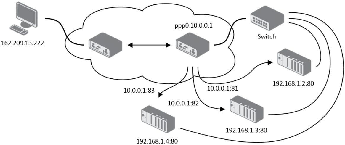
Figure 59: Topology for NAT Configuration Example 2
