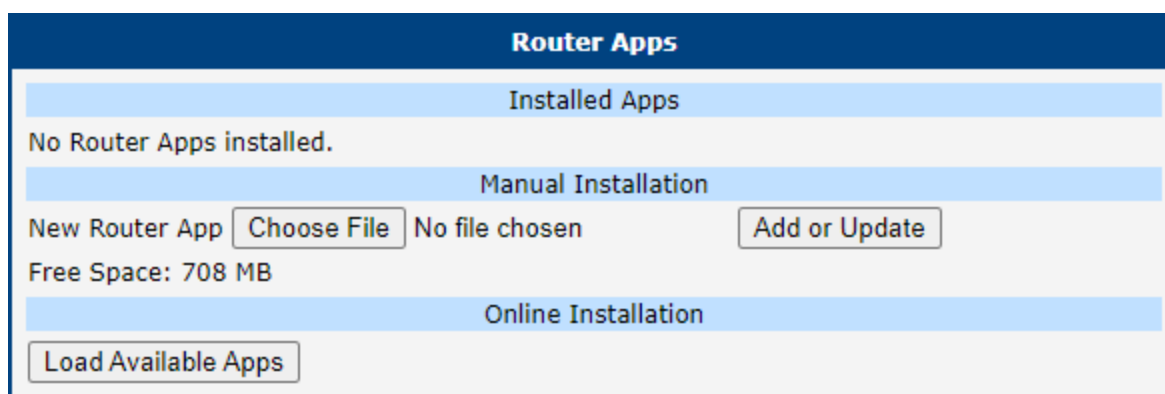
Figure 101: Default Router Apps GUI
