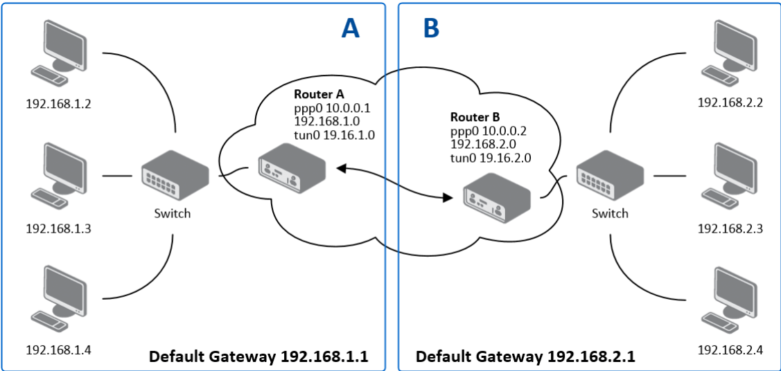
Figure 62: Topology of OpenVPN Configuration Example
