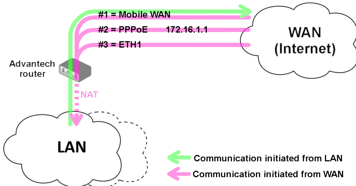
Figure 42: Example #3: Topology for Multiple WAN mode
