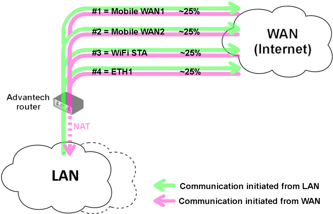
Figure 48: Example #6: Topology
