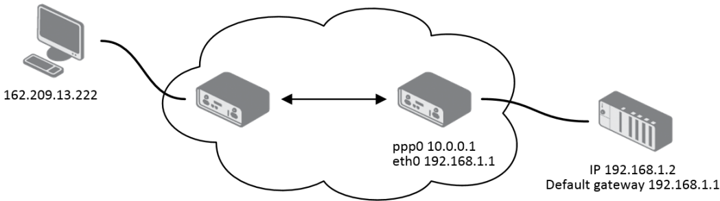
Figure 57: Topology for NAT Configuration Example 1
