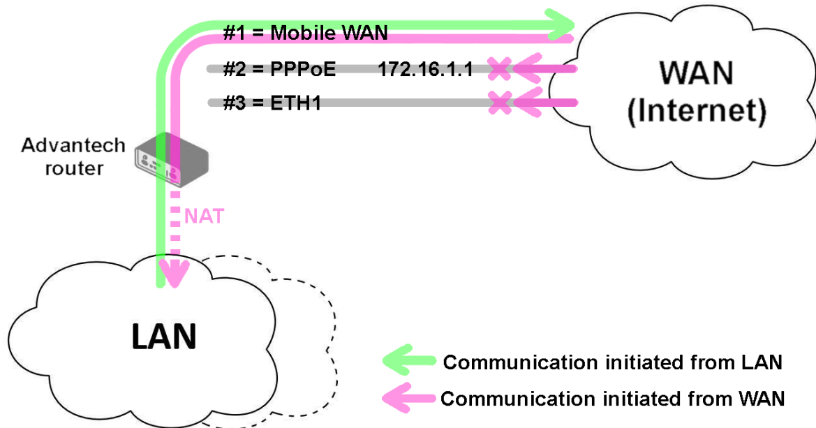
Figure 41: Example #3: Topology for Single WAN mode
