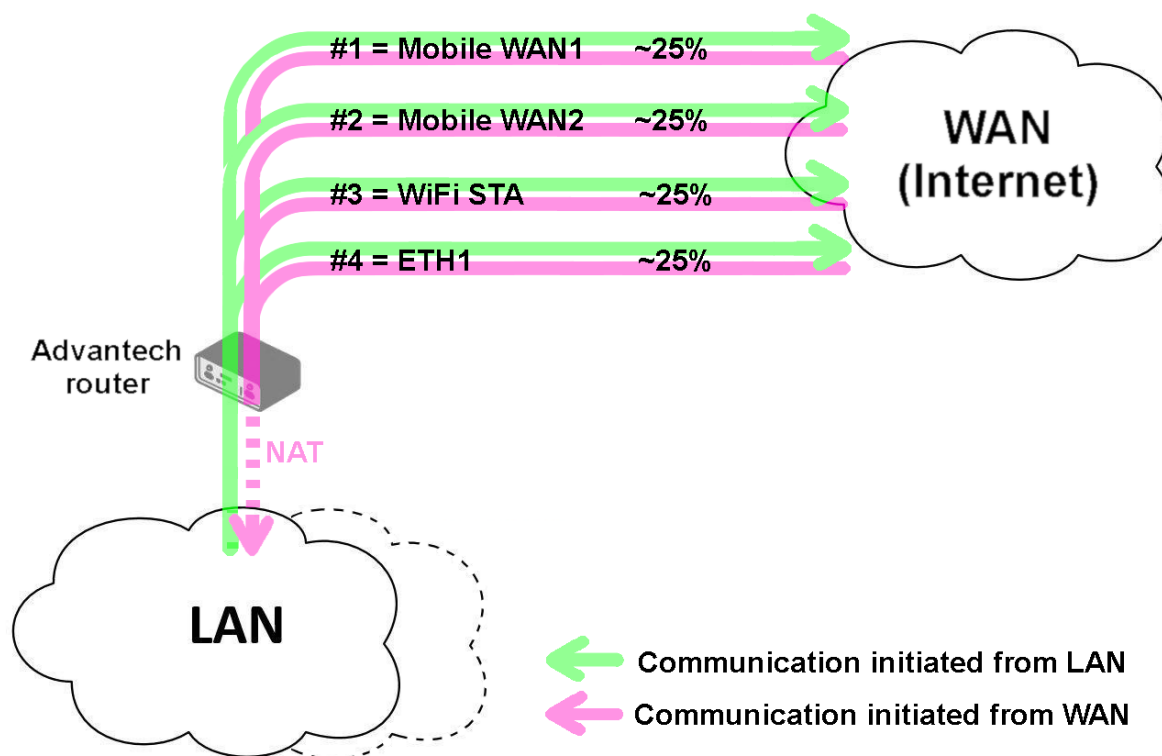
Figure 45: Example #6: Topology
