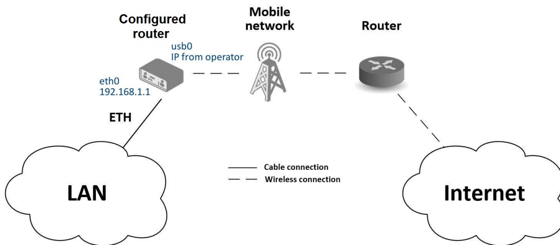
Figure 125: Access to the Internet from LAN – sample topology
