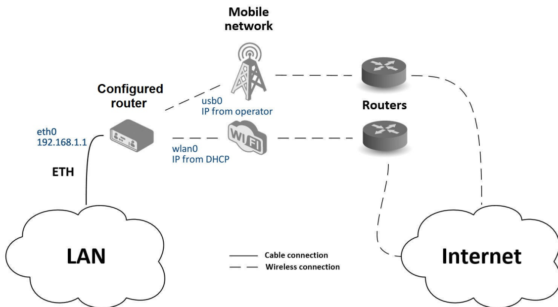
Figure 128: Backup access to the internet – sample topology
