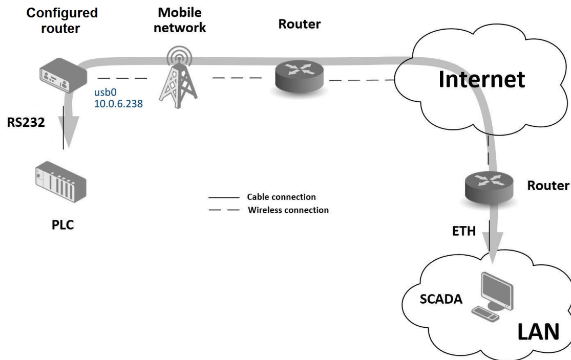
Figure 134: Serial gateway – sample topology
