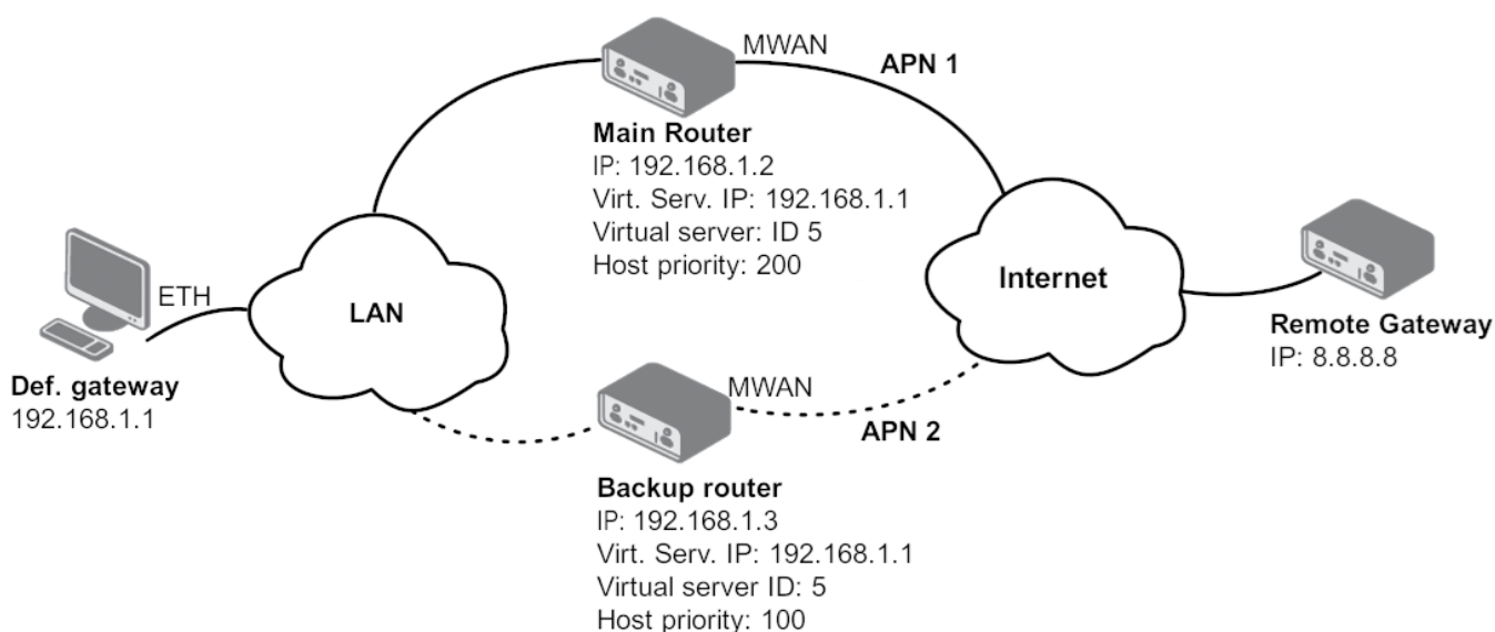
Figure 26: An example of VRRP topology
