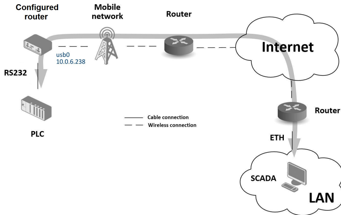
Figure 124: Serial Gateway – sample topology
