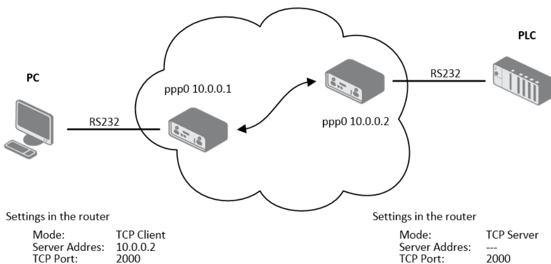
Figure 86: Example of serial interface extension
