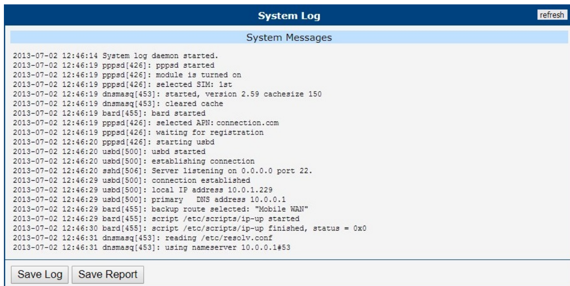
Figure 10: System Log
