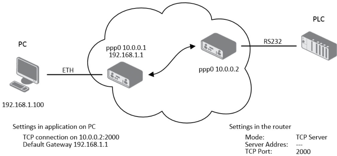
Figure 85: Example of Ethernet to serial communication
