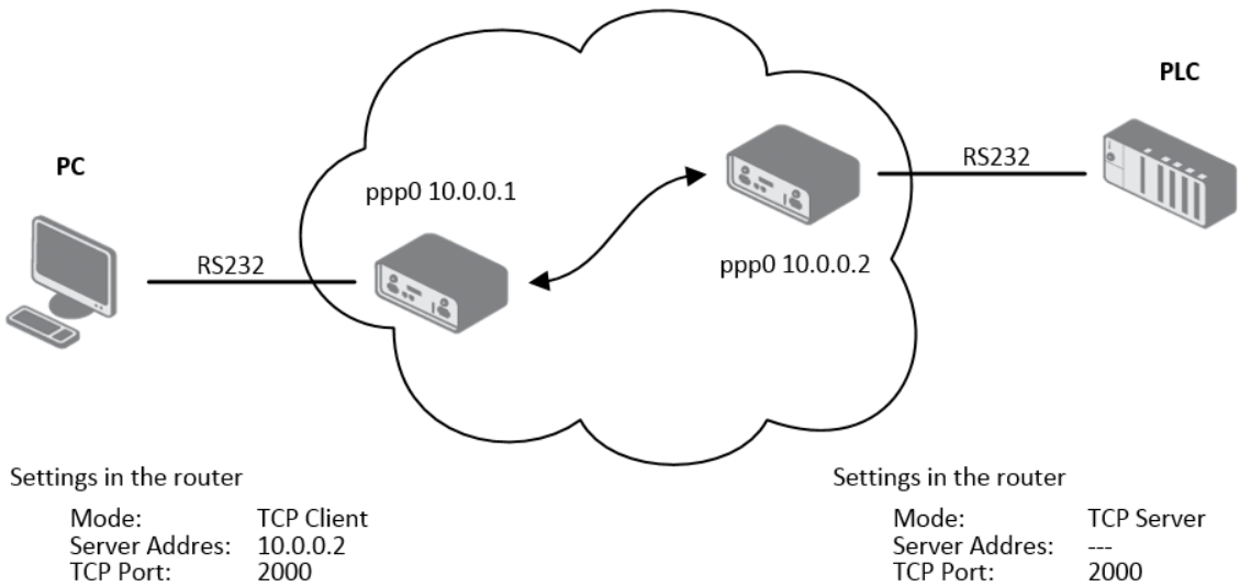
Figure 86: Example of serial interface extension
