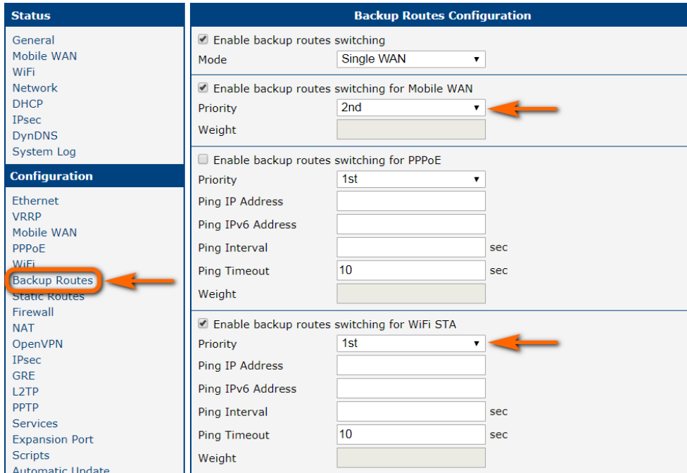
Figure 121: Backup access to the Internet – Backup Routes configuration
