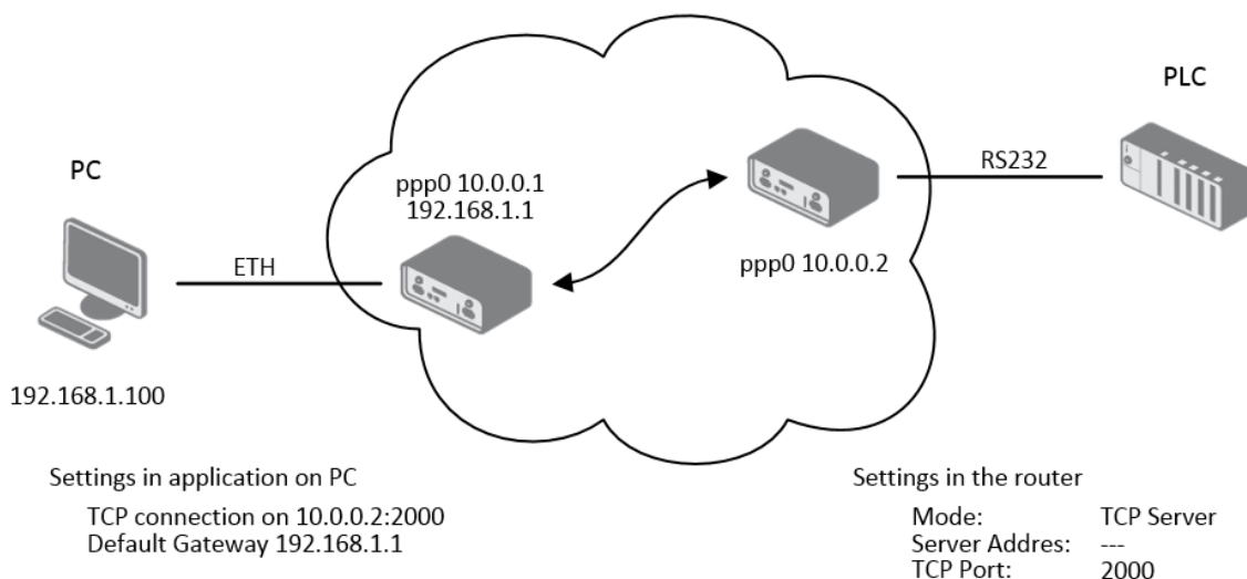
Figure 87: Example of Ethernet to serial communication
