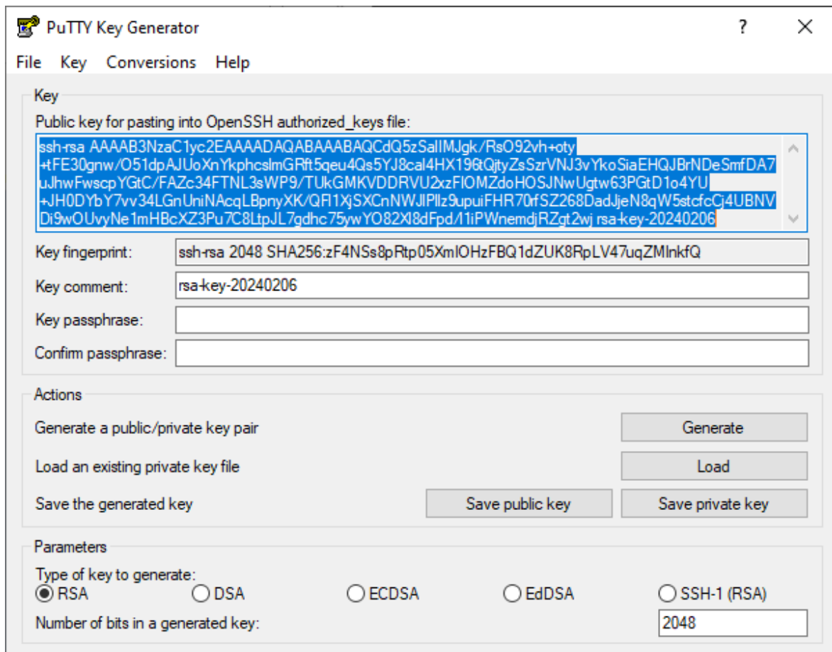
Figure 106: Key Generation
