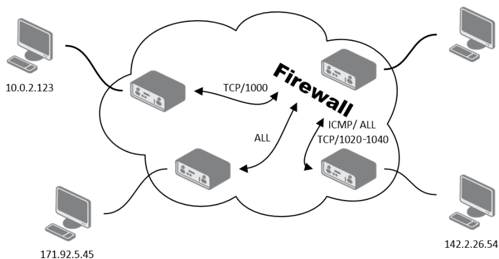
Figure 48: Topology for the IPv4 Firewall Configuration Example
