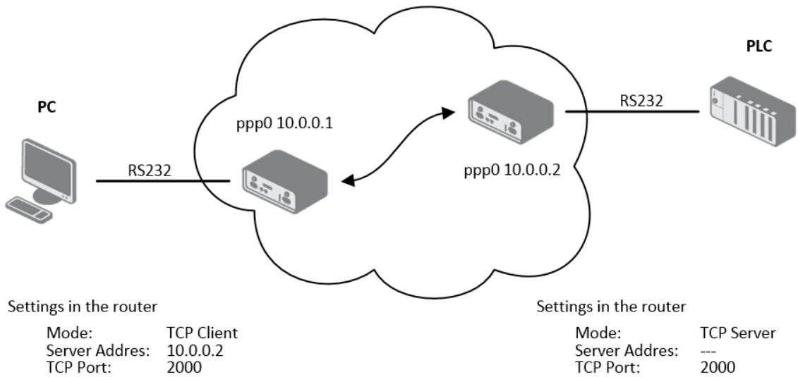
Figure 90: Example of serial interface configuration
