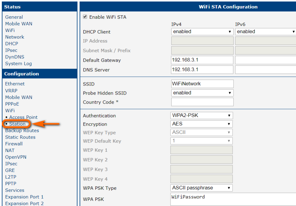
Figure 125: Backup access to the Internet – WiFi configuration
