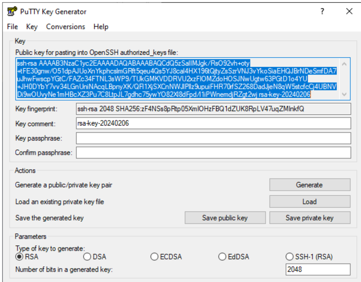
Figure 106: Key Generation
