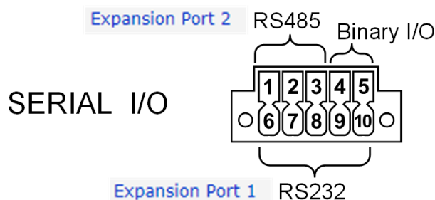
Figure 84: SERIAL I/O configuration pages overview
