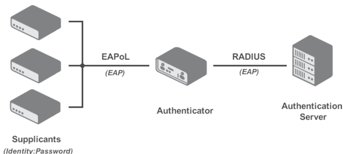
Figure 129: IEEE 802.1X Functional Diagram
