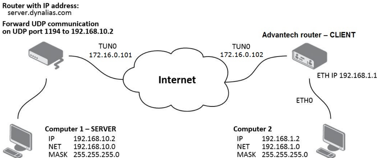
Figure 20: OpenVPN tunnel against Windows/Linux SERVER
