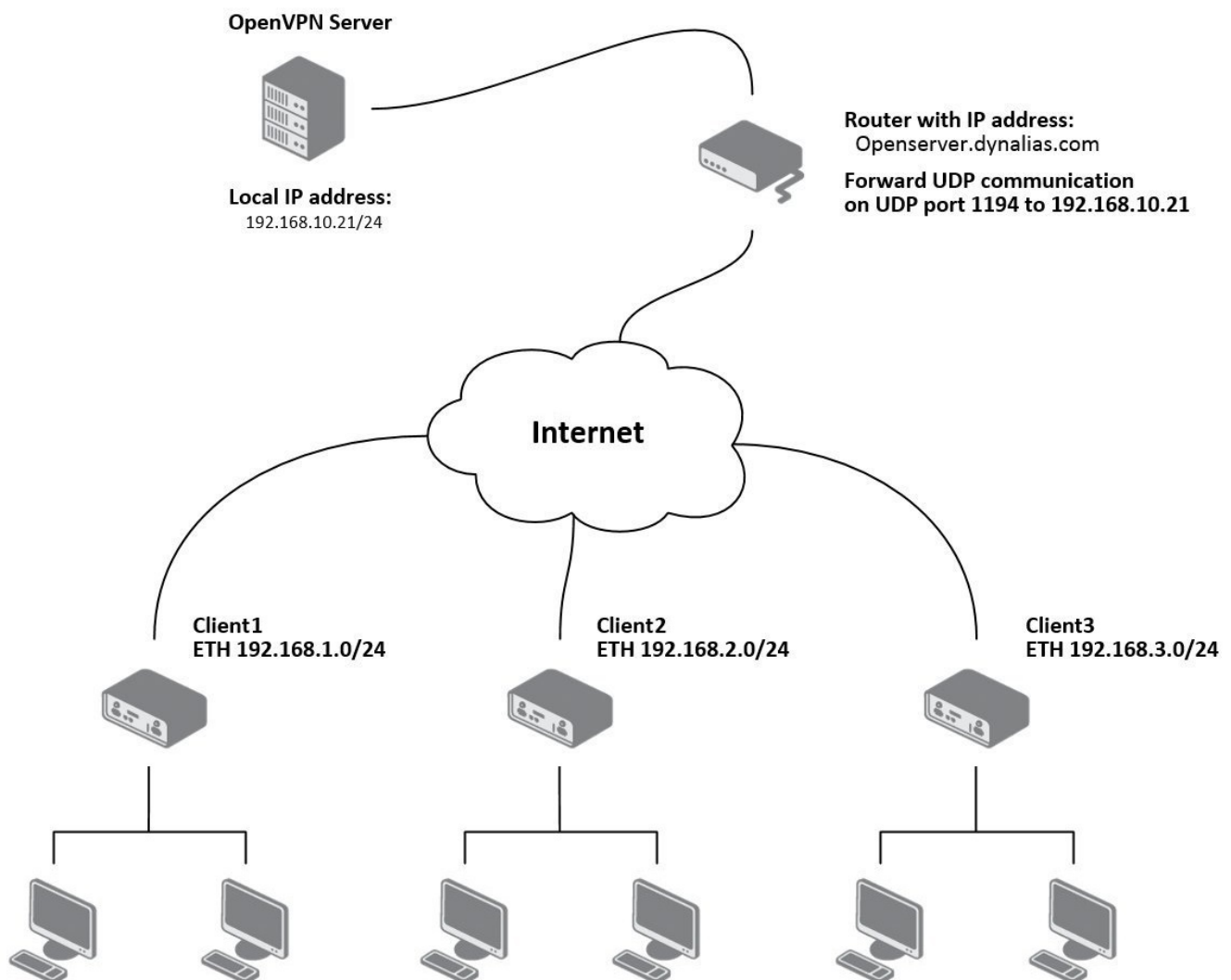
Figure 26: OpenVPN client to client
