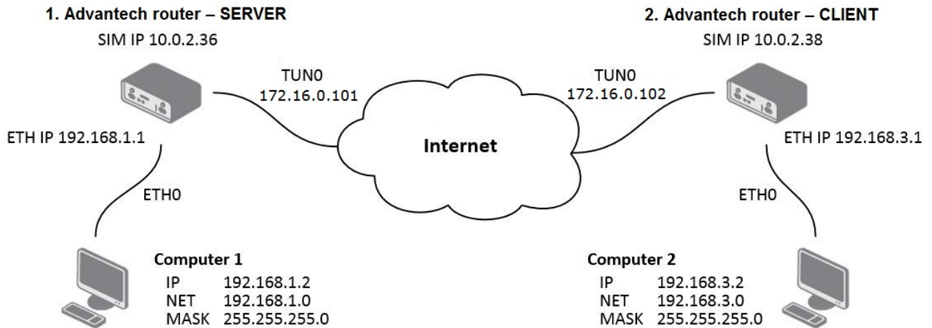
Figure 3: Router on both sides of tunnel
