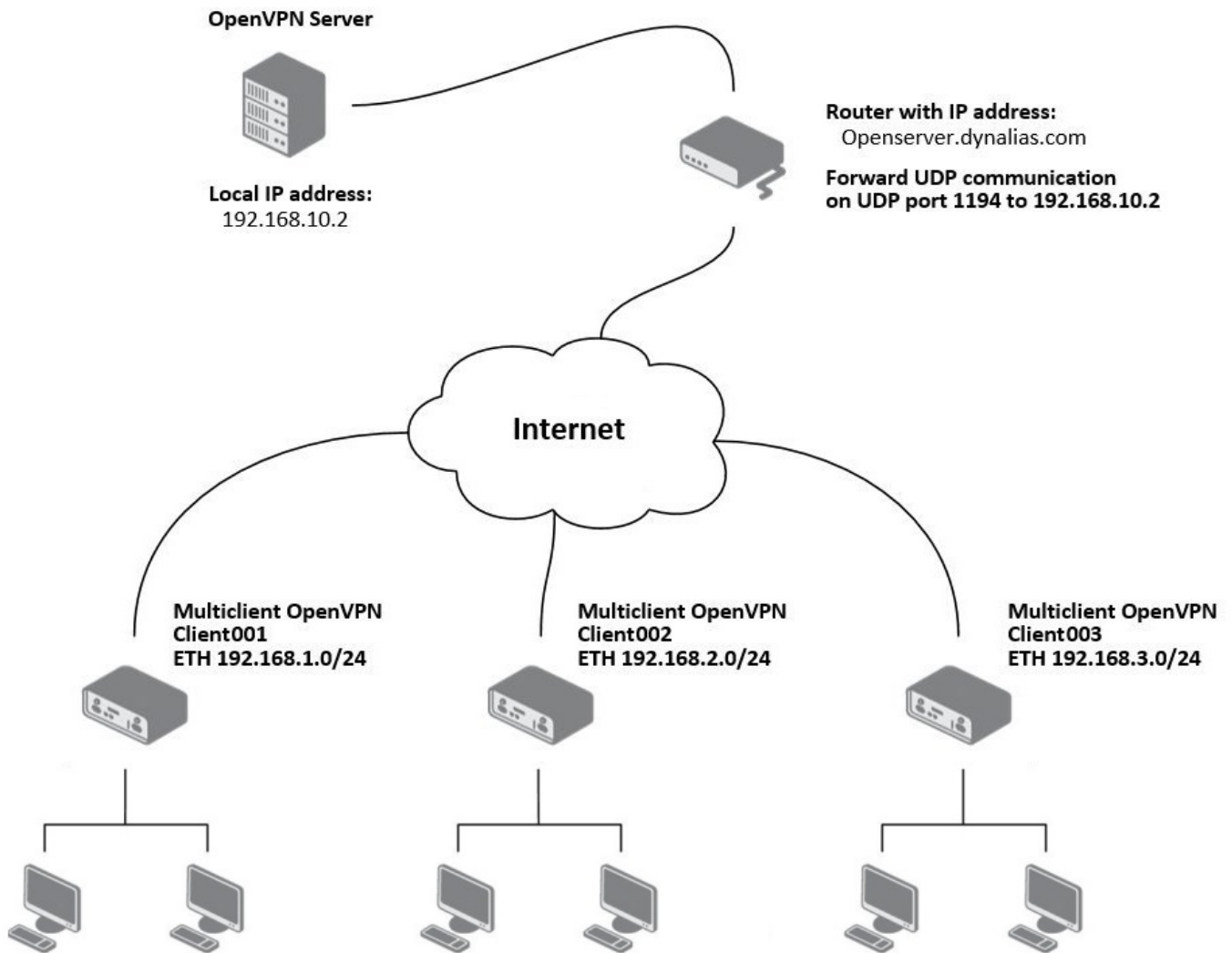
Figure 24: OpenVPN Multiserver – Advantech router (CLIENT)
