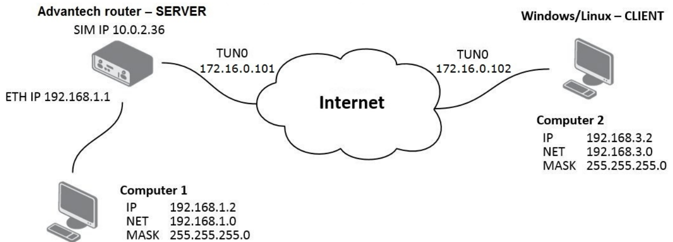
Figure 16: OpenVPN tunnel against Windows/Linux CLIENT
