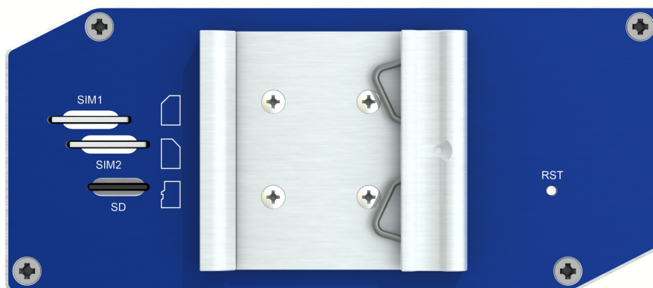
Figure 2: BB-SBD45 DIN Bracket on SmartFlex Router
