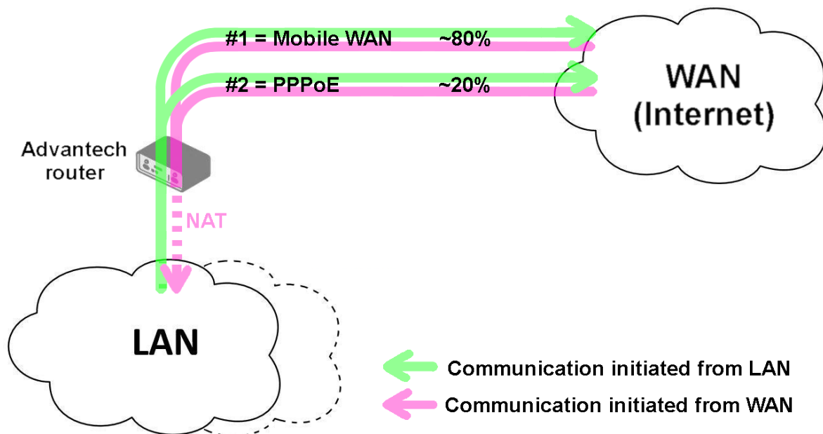
Figure 40: Example #4: Topology
