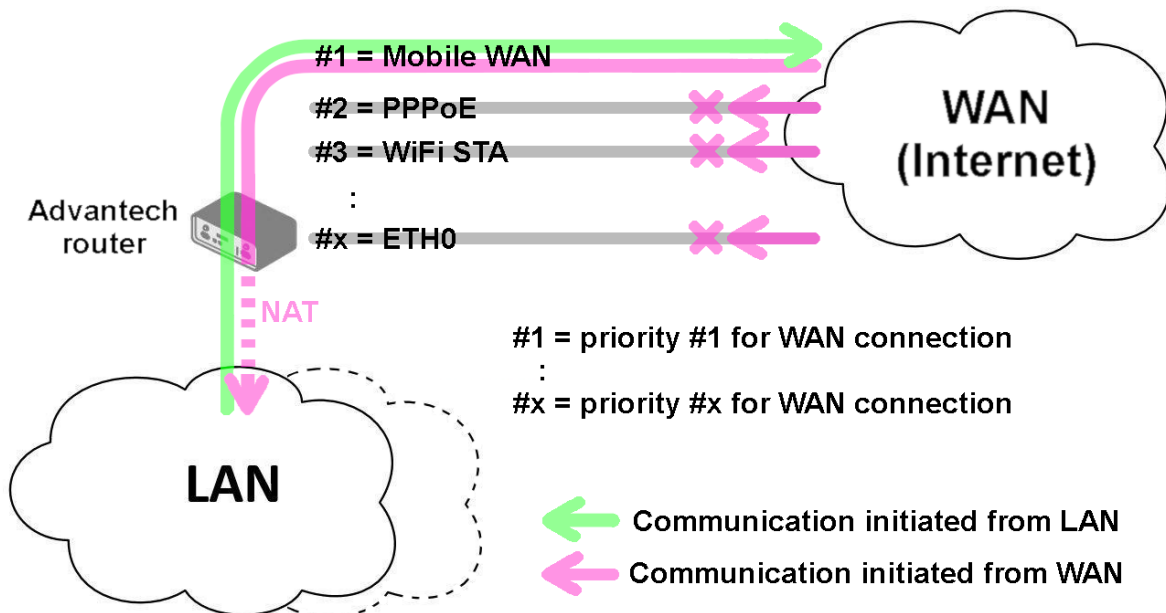
Figure 33: Example #1: Topology
