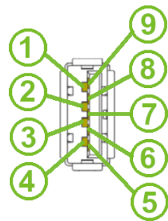
Figure 17: USB 3.0 connector pinout
