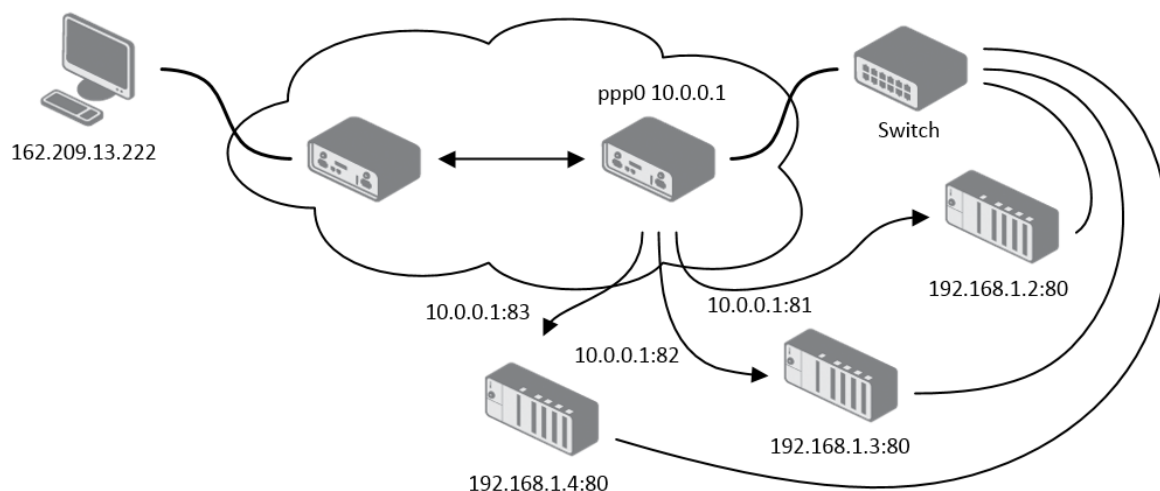
Figure 49: Topology for NAT Configuration Example 2
