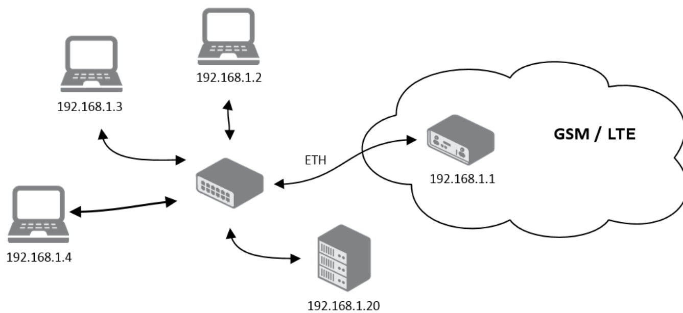
Figure 18: Network topology for example 1
