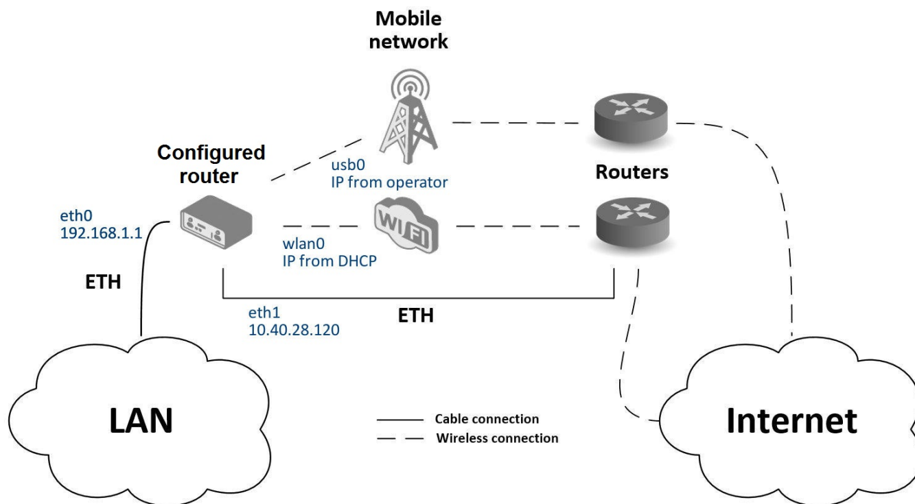
Figure 124: Backup access to the internet: a topology example
