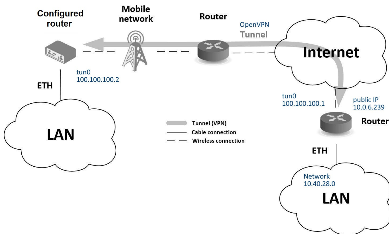
Figure 129: Secure networks interconnection: a topology example
