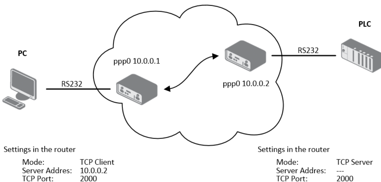
Figure 88: Example of Serial Interface Configuration
