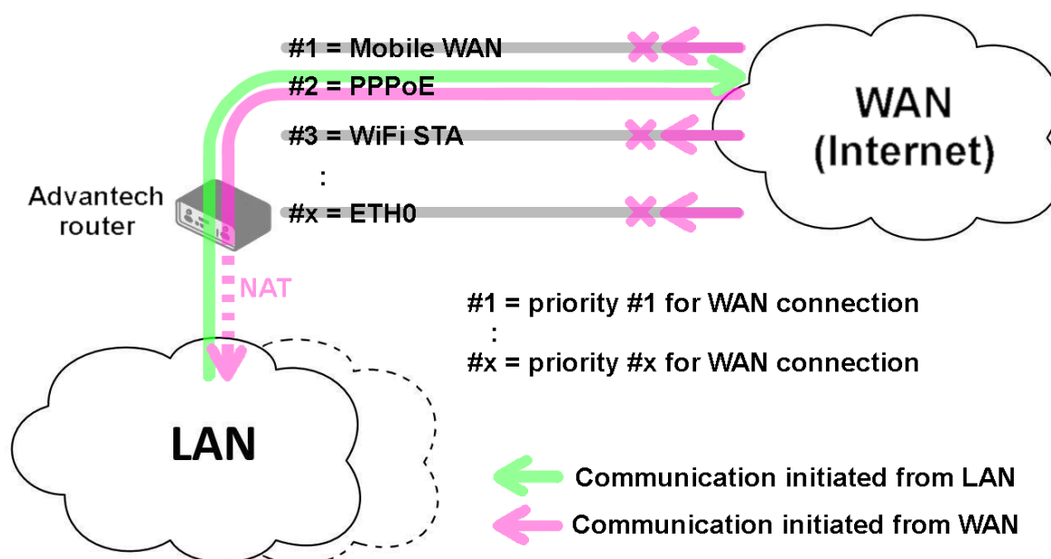
Figure 36: Example #2: Topology
