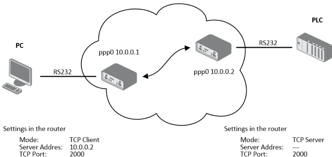
Figure 88: Example of serial interface configuration
