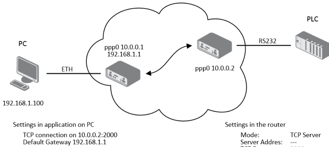
Figure 87: Example of Ethernet to serial communication configuration
