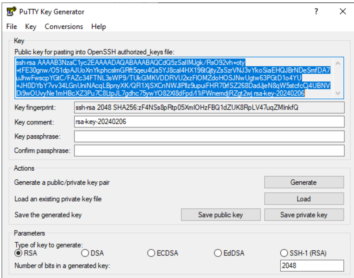
Figure 105: Key Generation
