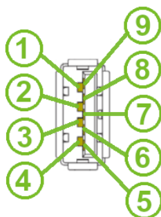
Figure 13: USB 3.0 Connector Pinout
