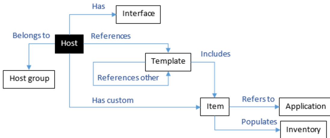
Figure 1: Logical Schema of a Zabbix Configuration
