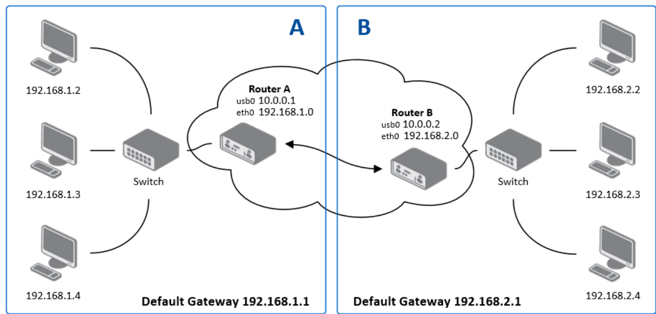
Figure 65: IPsec configuration topology example
